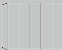
Hinged-door wardrobes doors in carcass colour, coloured glass or mirrored glass, W 50 – 400 cm, H 216 cm, D 58 cm
