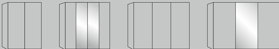
Sliding-door wardrobes wooden doors in carcase colour and 1-3 mirrored doors W 150, 200, 250 and 300 cm, H 217cm, D 67 cm
